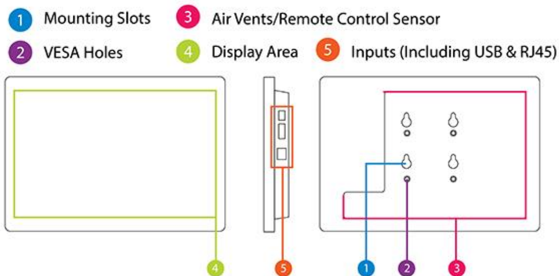
Figure 2 Product Overview
